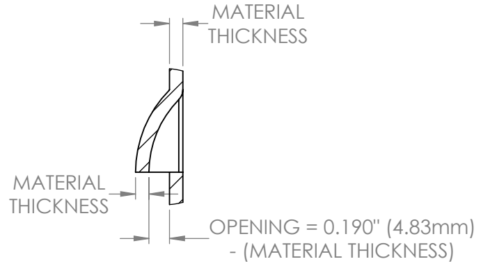
DETAIL A SCALE 2 : 1.5
